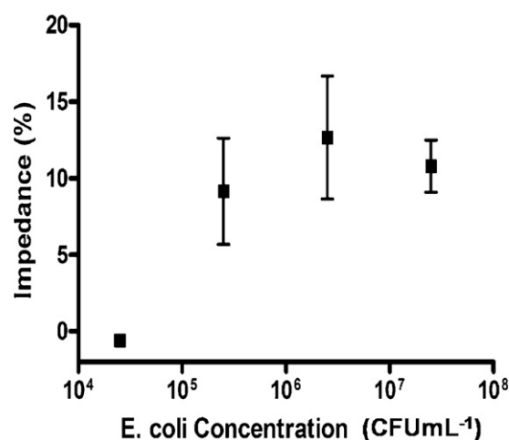
Fig. 6. Graph showing the relation between the concentrations of the E. coli vs. impedance (%) (dose response).
