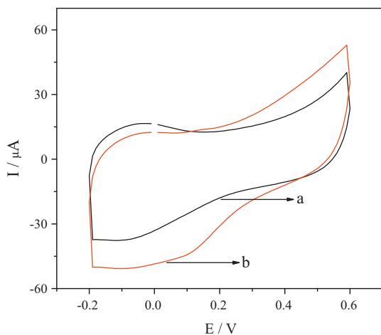
Fig. 5. CVs of the biosensor in 0.05 M PBS (pH 7.0) without cholesterol (a) and with 0.6 mM cholesterol (b) at the scan rate of 50 \text{ mV s}^{-1} .
