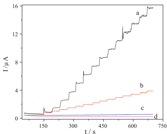
Fig. 7. Typical current–time response curves of different modified electrodes for successive addition of 40 \mu\text{M} cholesterol. (a) ChOx/Pt–Au@ZnONRs/CS–MWCNTs/GCE, (b) ChOx/Pt–Au@ZnONRs/GCE, (c) ChOx/CS–MWCNTs/GCE and (d) CS–ChOx/GCE. Test solution: stirring 0.05 M pH 7.0 PBS. Applied potential: 0.45 V.
