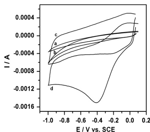
Fig. 3. Cyclic voltammograms of bare graphite (a, b) and FG/Gr electrode (c, d) in the absence of (a, c) and presence of (b, d) 6 mM \text{H}_2\text{O}_2 in 0.1 M PBS (pH 7.0) scan rate 25 \text{ mVs}^{-1} .
