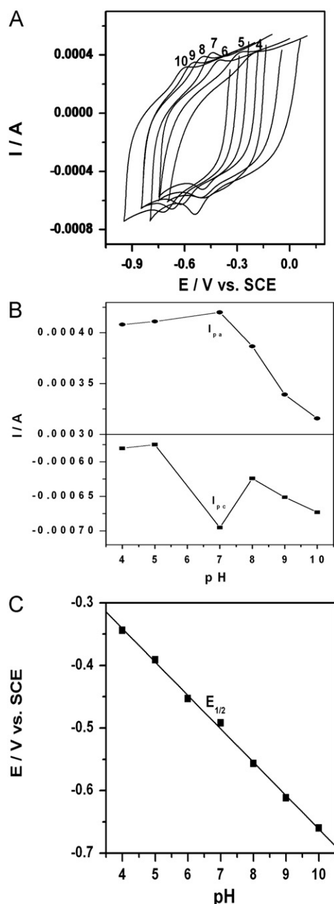
Fig. 7. (A) CVs of ChOx-FG/Gr electrode at various pHs of the solution (pH 4–10) scan rate: 100\text{ mVs}^{-1} . (B) Relationship between anodic peak current ( I_{pa} ), cathodic peak current ( I_{pc} ) with pH.
