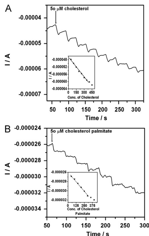
Fig. 8. (A) Amperometric response of ChOx-FG/Gr electrode for each addition of 50\text{ }\mu\text{M} cholesterol at constant applied potential -350\text{ mV} in PBS containing 0.1\text{ M} KCl (pH 7.0). Inset shows relationship between cathodic peak current ( I_{pc} ) and concentrations of cholesterol. (B) Amperometric response of (ChEt/ChOx)-FG/Gr electrode for each addition of 50\text{ }\mu\text{M} cholesterol palmitate at constant applied potential -350\text{ mV} in PBS containing 0.1\text{ M} KCl (pH 7.0). Inset shows relationship between cathodic peak current ( I_{pc} ) and concentrations of cholesterol palmitate.
