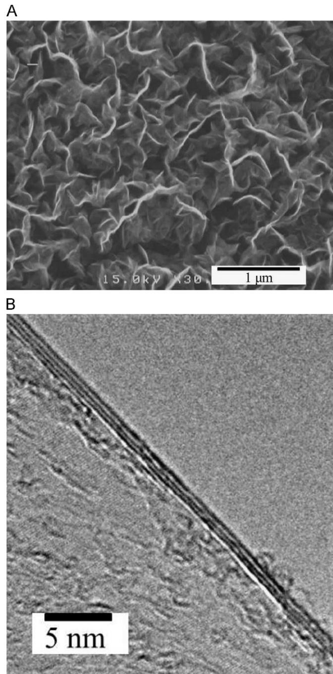
Fig. 1. (A) SEM and (B) TEM images of the CNS films grown on the Cu surface by MPECVD.
