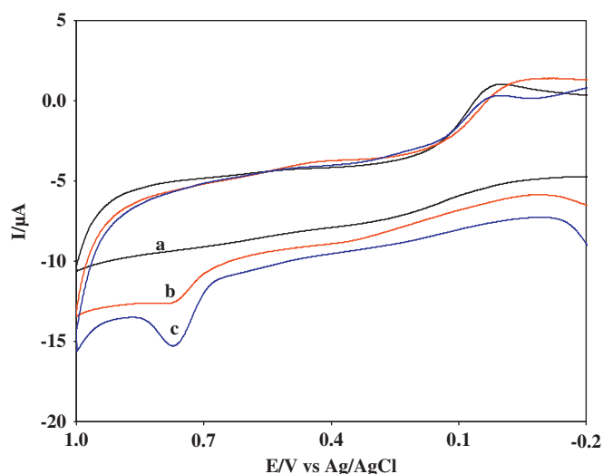
Fig. 7. Typical electrochemical response of the SOD1-CNT-PPy-Pt electrode for endothelial cells treated with (a) control, (b) 250 \mu\text{M} \text{H}_2\text{O}_2 and (c) 500 \mu\text{M} \text{H}_2\text{O}_2 in 0.1 M PBS (pH 7.0) at scan rate: 100 \text{mV s}^{-1} vs. Ag/AgCl.
