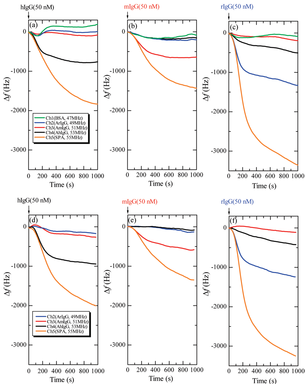
Figure 5. Resonance frequency changes caused by the injection of (a) 50 nM hIgG, (b) 50 nM mIgG, and (c) 50 nM rIgG solutions. Parts d–f are frequency changes of the four channels, where the response of the reference channel (BSA channel) is subtracted.
