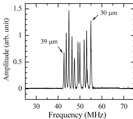
Figure 2. Resonance spectrum from 10-channel quartz plates with different thicknesses between 30 and 39 \mu\text{m} immersed in PBS measured by the line antenna wires contactlessly.
