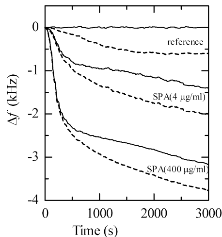
Figure 4. Frequency changes of the three-channel WE-MQCM caused by the injection of a 515 nM hIgG solution (broken lines). The reference channel indicates the quartz plate covered by BSA through the SAM. The other two channels are SPA-immobilized quartz plates. The concentration values indicate the SPA concentrations in the immobilization process. The solid lines are frequency changes, where the reference channel response is subtracted.
