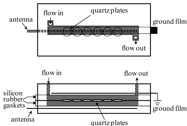
Figure 1. Schematic of the multichannel sensor cell. The two antenna wires are embedded in the bottom Teflon block, and the thin grounding foil is in the top Teflon block. The silicon rubbers lightly grasp parts of the edges of the quartz plates.
