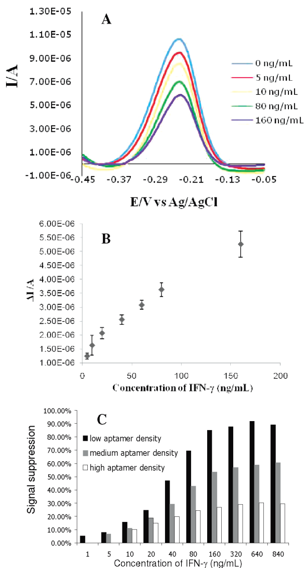
Figure 3. Characterization of sensor response to IFN- \gamma . (A) Voltammograms obtained with SWV showed that decrease in faradaic current was proportional to solution concentration of IFN- \gamma . These results were obtained with gold electrodes modified with 2 \mu M concentration of aptamer (medium aptamer density). (B) Calibration curve of current vs IFN- \gamma concentration for aptasensor prepared using 2 \mu M aptamer concentration. The calibration curve was fitted to a line with the equation of y = 2 \times 10^{-8}x + 1 \times 10^{-6} and R^2 of 0.9801. The data points and error bars represent average and standard deviations of measurements from three different aptamer-modified electrodes ( n = 3 ). (C) Sensitivity of electrodes with different aptamer packing densities was expressed as the loss or suppression of signal (current) upon binding of 50 nM IFN- \gamma . The larger the signal suppression (or current loss), the higher is the sensitivity of the biosensor. Electrodes with low, medium, and high packing density were prepared using 0.5, 2, and 8 \mu M aptamer concentrations. Aptasensors with low packing density were found to be most sensitive with a detection limit of 0.06 nM or 1 ng/mL IFN- \gamma .
