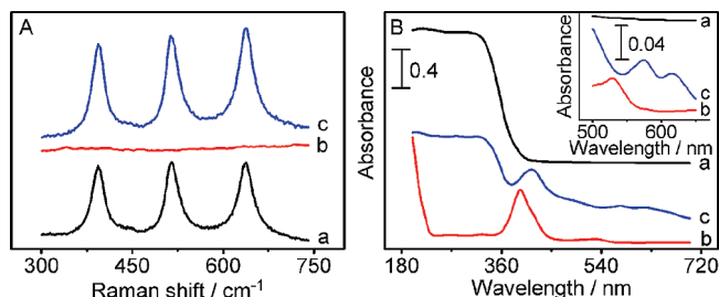
Figure 2. (A) Raman and (B) UV–vis absorption spectra of (a) TiO 2 , (b) FeTPPS, and (c) FeTPPS-TiO 2 powders. Inset: amplified UV–vis absorption spectra.
