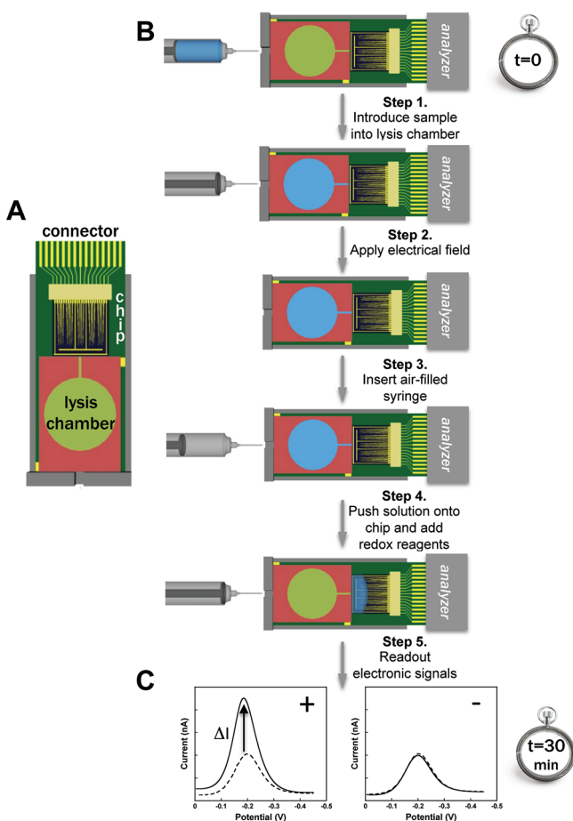
Figure 2. Integrated sensing system. (A) Schematic of cartridge integrating lysis chamber, NME chip, and connector to analyzer. (B) Overview of detection scheme; injection, lysis, delivery, and readout in 30 min. (C) Typical differential pulse voltammograms of positive (left) and negative (right) samples where the dotted line is the background and the solid line is the readout.
