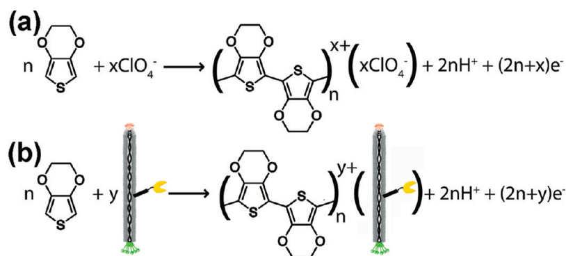
Scheme 1. (a) Electrochemical Oxidation of EDOT to Form PEDOT in Perchlorate-Containing Electrolyte. (b) Electrochemical Oxidation of EDOT in the Presence of Negatively-Charged M13 Virus Particles to Form PEDOT a
