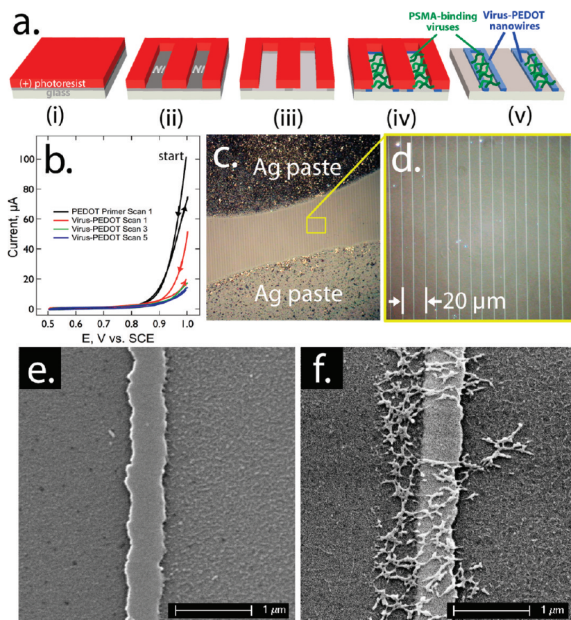
Figure 2. Synthesis of virus–PEDOT nanowires: (a) Process flow for the preparation, using the LPNE process, of virus–PEDOT composite nanowires for the detection of PSMA. (b) Cyclic voltammograms for the electrodeposition of virus–PEDOT nanowires within the LPNE microfabricated template. Two primer scans were first carried out in aqueous 2.5 mM EDOT, 12.5 mM LiClO 4 (black). Then, five additional scans in 2.5 mM EDOT, 10 nM PSMA-binding viruses, and 12.5 mM LiClO 4 were used to build up a virus–PEDOT composite nanowire 200–300 nm in total width. (c,d) Optical micrographs of the resulting nanowire array on glass after the application of silver paste electrical contacts. (e,f) Scanning electron micrographs of single nanowires of pure PEDOT (e) and the virus–PEDOT composite (f). The net-like structures observed in (f) are aggregates of filamentous M13 virus particles.
