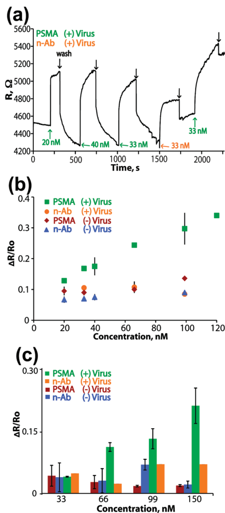
Figure 4. Real-time biosensing with PSMA-binding PEDOT nanowires. (a) A real-time trace of biosensing data, with the indicated injections of negative antibody (n-Ab), PSMA, or washes with PBF buffer (black arrows). (b) A compilation of all real-time biosensing data, depicted as a calibration curve with error bars indicating standard deviation ( n = 3 ). The change in resistance upon injection is plotted versus analyte concentration. (c) A plot demonstrating the change in resistance upon injection of analytes in a solution of synthetic urine (errors bars indicate standard deviation with n = 3 ).
