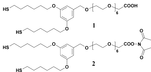
Chart 1. Structure of Dithiols Used in This Work
