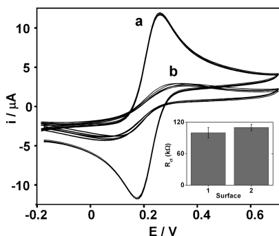
Figure 2. Typical overlay of cyclic voltammograms (in 1 mM \text{K}_3\text{Fe}(\text{CN})_6 in 0.1 M KCl) obtained with the electrode array at bare gold (a) and SAM of 2 (b). Inset: Impedance responses obtained after derivatization of the surface with anti-CEA antibody at SAMs of 1 and 2 .
