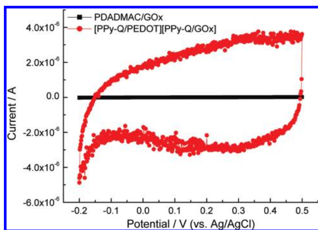
FIGURE 4. CV of functionalized gold electrodes with two different LbL film compositions.
