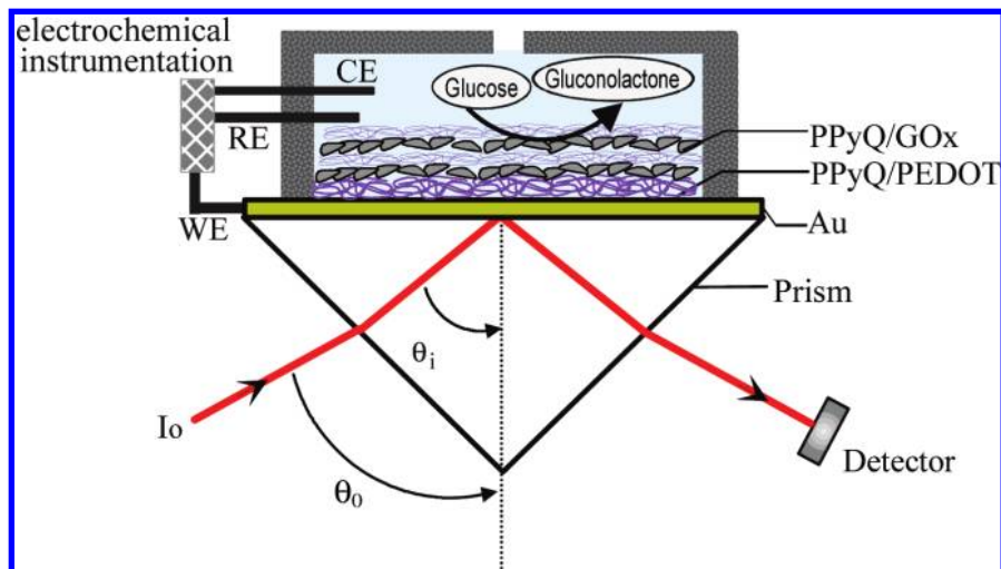
FIGURE 1. EC-SPR glucose biosensor schematic diagram in a Kretschmann configuration with a three-electrode cell setup.
