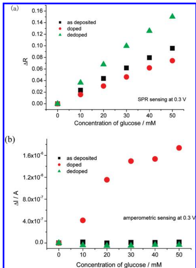
FIGURE 6. Plot of amperometric vs SPR sensing with an increase in the concentration of glucose.
