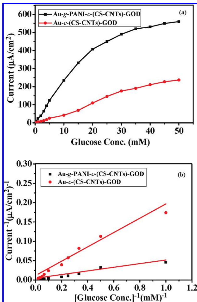
FIGURE 8. (a) Glucose concentration ( C_{\text{glucose}} ) dependence of the response current ( i ) for the Au- g -PANI- c -(CS-CNTs)-GOD and Au- c -(CS-CNTs)-GOD electrodes, and (b) the Lineweaver–Burk plots of (1/i_{ss})^{-1} vs (1/C_{\text{glucose}})^{-1} , where i_{ss} is the steady-state current.
