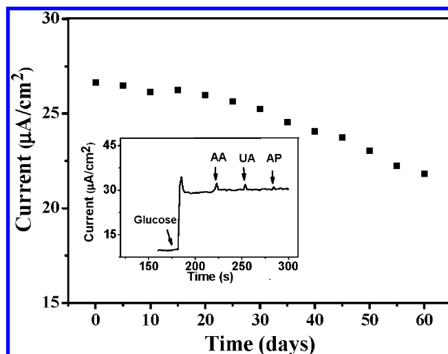
FIGURE 9. Response current ( C_{\text{glucose}} = 10 \text{ mM} ) of the Au- g -PANI- c -(CS-CNTs)-GOD electrode as a function of storage time. The inset shows the amperometric responses of the Au- g -PANI- c -(CS-CNTs)-GOD electrode to glucose (1.0 mM), in the presence of ascorbic acid (AA, 0.3 mM), uric acid (UA, 0.3 mM), and acetaminophen (AP, 0.3 mM) in PBS (pH 6.0) at an applied potential of 0.5 V.
