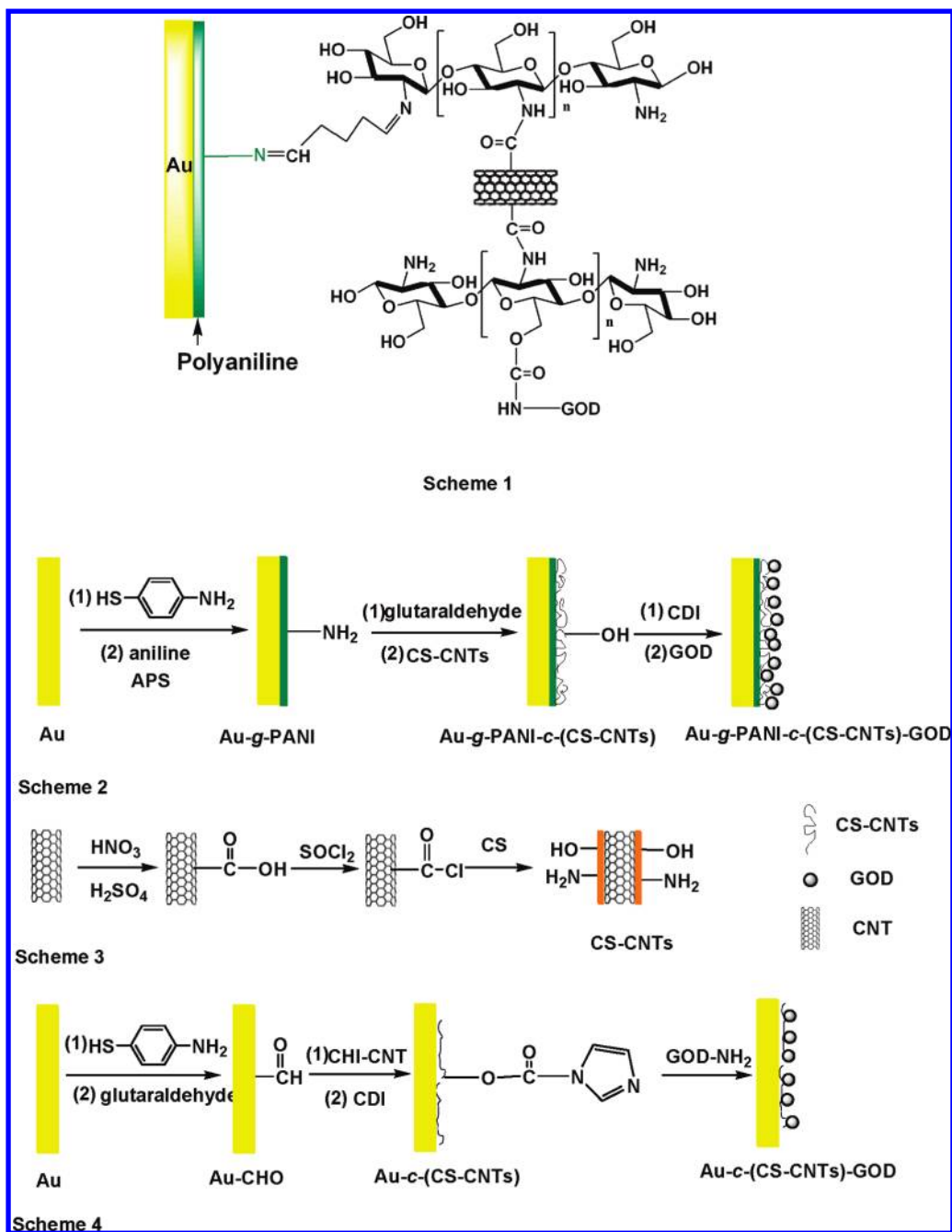
FIGURE 1. Schematic diagrams illustrating the process of fabrication of the Au-g-PANI-c-(CS-CNTs)-GOD (Schemes 1–3), and Au-c-(CS-CNTs)-GOD (Scheme 4) biosensors.
