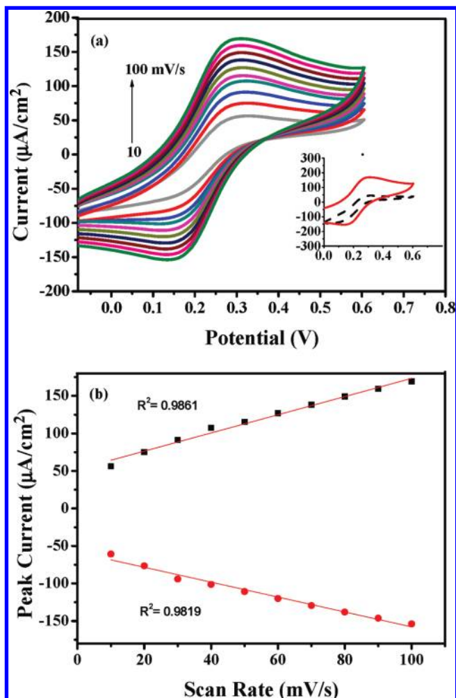
FIGURE 6. (a) Cyclic voltammograms (CVs) of the Au- g -PANI- c -(CS-CNTs)-GOD electrode at scan rates of 10, 20, 30, 40, 50, 60, 70, 80, 90, and 100 mV/s in 1 mM PBS (pH 6.0) of \text{Fe}(\text{CN})_6^{3-/4-} under a nitrogen atmosphere. The inset is the CVs of Au- c -(CS-CNTs)-GOD (dash line) and Au- g -PANI- c -(CS-CNTs)-GOD (solid line) electrodes at the scan rate of 100 mV/s. (b) Dependence of peak currents on scan rates.
