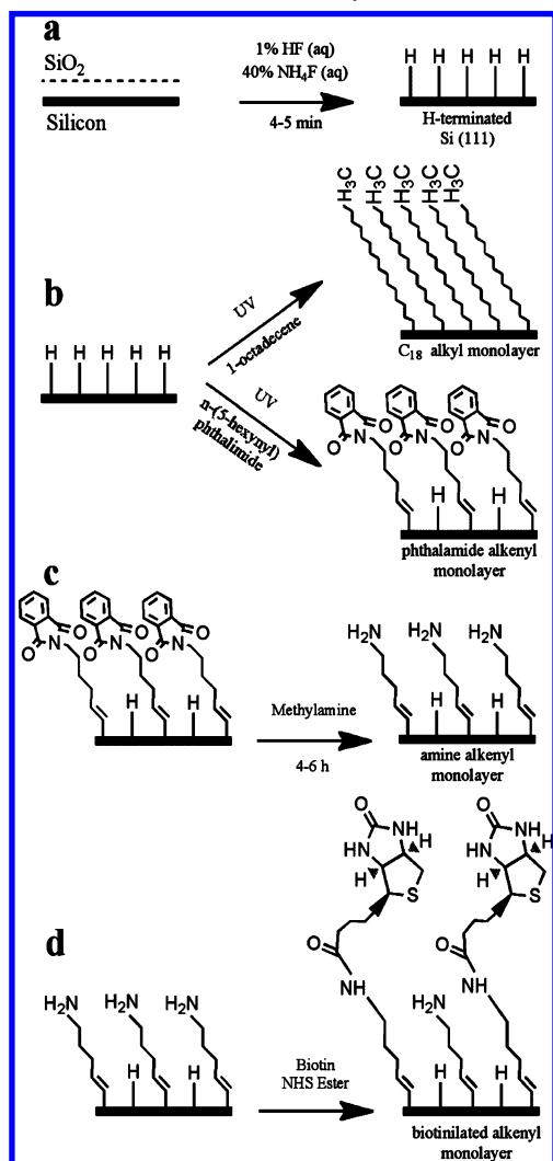
(a) Si–H surface formation: remove native \text{SiO}_2 with 1% HF (aq) followed by surface preparation with 40% \text{NH}_4\text{F} (aq). (b) Hydrosilylation UV reaction forming \text{C}_{18} alkyl and phthalimide alkenyl monolayers. (c) Deprotection of amine terminal groups. (d) Conjugate biotin to amine groups.
