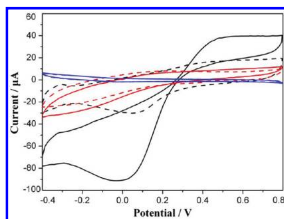
Figure 7. Cyclic voltammograms of GC/BNNTs-Pt (red) GC/BNNTs-Pani (blue) and GC/BNNTs-Pani-Pt (black) electrodes obtained in the absence (dotted line) and presence (solid line) of 5 mM \text{H}_2\text{O}_2 in 0.2 M PBS solution at 50 \text{mV s}^{-1} (vs SCE).
