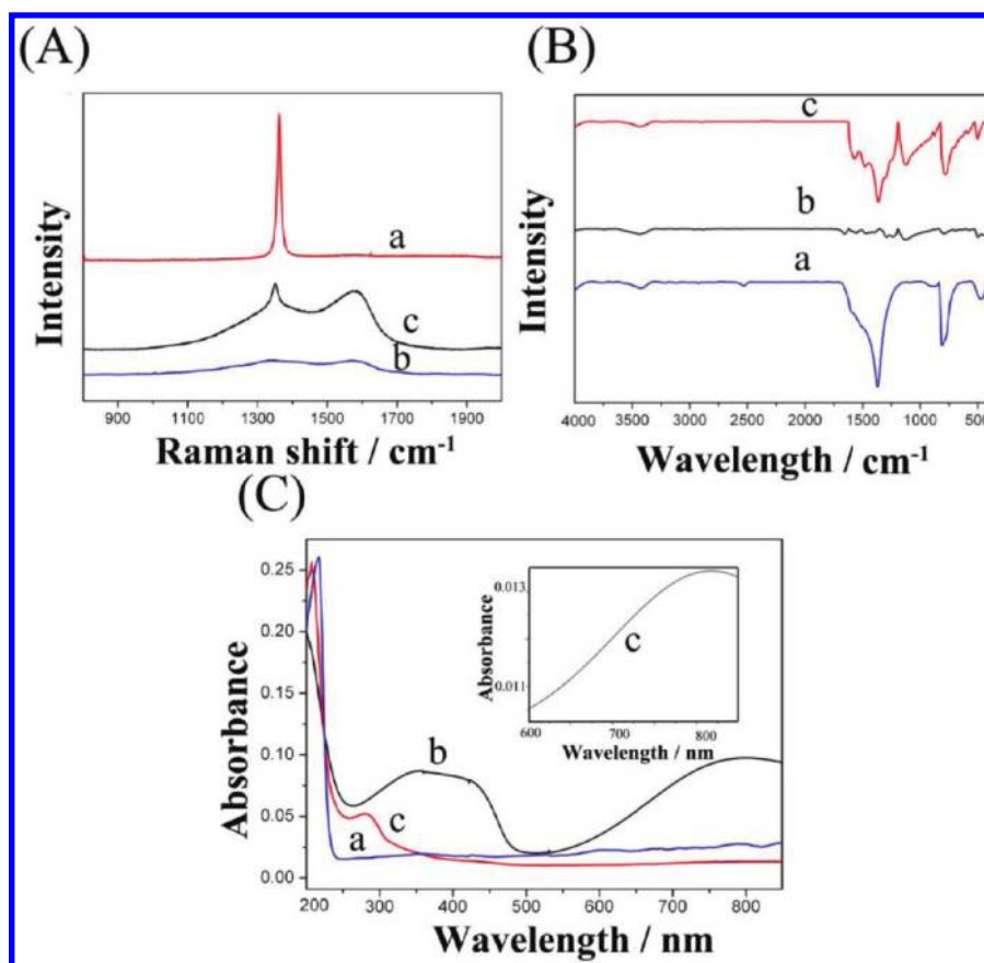
Figure 3. (A) Raman, (B) FT-IR, and (C) UV-vis absorption spectra of (a) BNNTs, (b) Pani, and (c) BNNTs-Pani hybrids.
