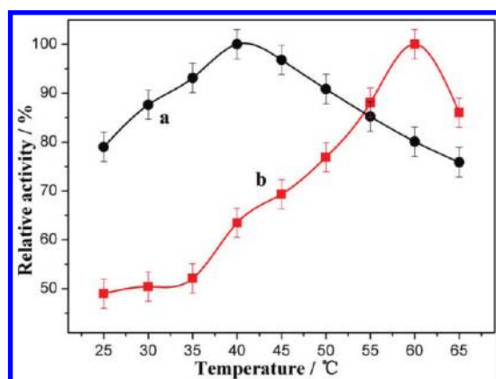
Figure 11. Contrastive study of the effect of temperature on the activities of (a) GC/Pani-Pt-GOD and (b) GC/BNNTs-Pani-Pt-GOD electrodes.
