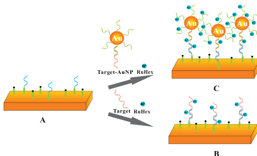
FIGURE 3. Scheme for an AuNP-amplified chronocoulometric DNA sensor.
