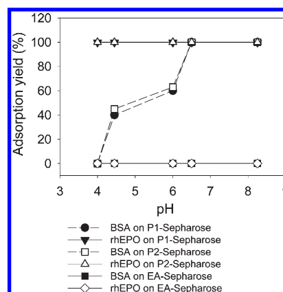
Figure 3. Influence of pH on rhEPO and BSA adsorption to peptide-Sepharose and ethanolamine (EA)-Sepharose. Samples of rhEPO and BSA in 20 mM sodium phosphate buffers with pHs from 4.00 to 8.25 were loaded on columns ( 0.5 \times 5 \text{ cm} ) filled with EA-Sepharose, P1-Sepharose, or P2-Sepharose. The columns were washed with the equilibrating buffer at a flow rate of 0.25 \text{ mL/min} until the absorbance at 280 nm reached its initial value. Thereafter, the elution of the bound protein was accomplished with 100 mM sodium acetate buffer, pH 3.0, 0.25 M NaCl at the same flow rate.
