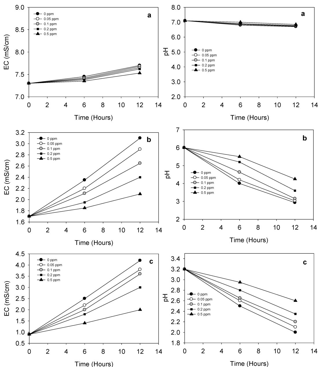
Figure 3. EC and pH values of media containing alkalinities of (a) 1567, (b) 293, and (c) 17.5 mg/L as CaCO 3 and NO 2 - concentrations of 0–0.5 ppm.
