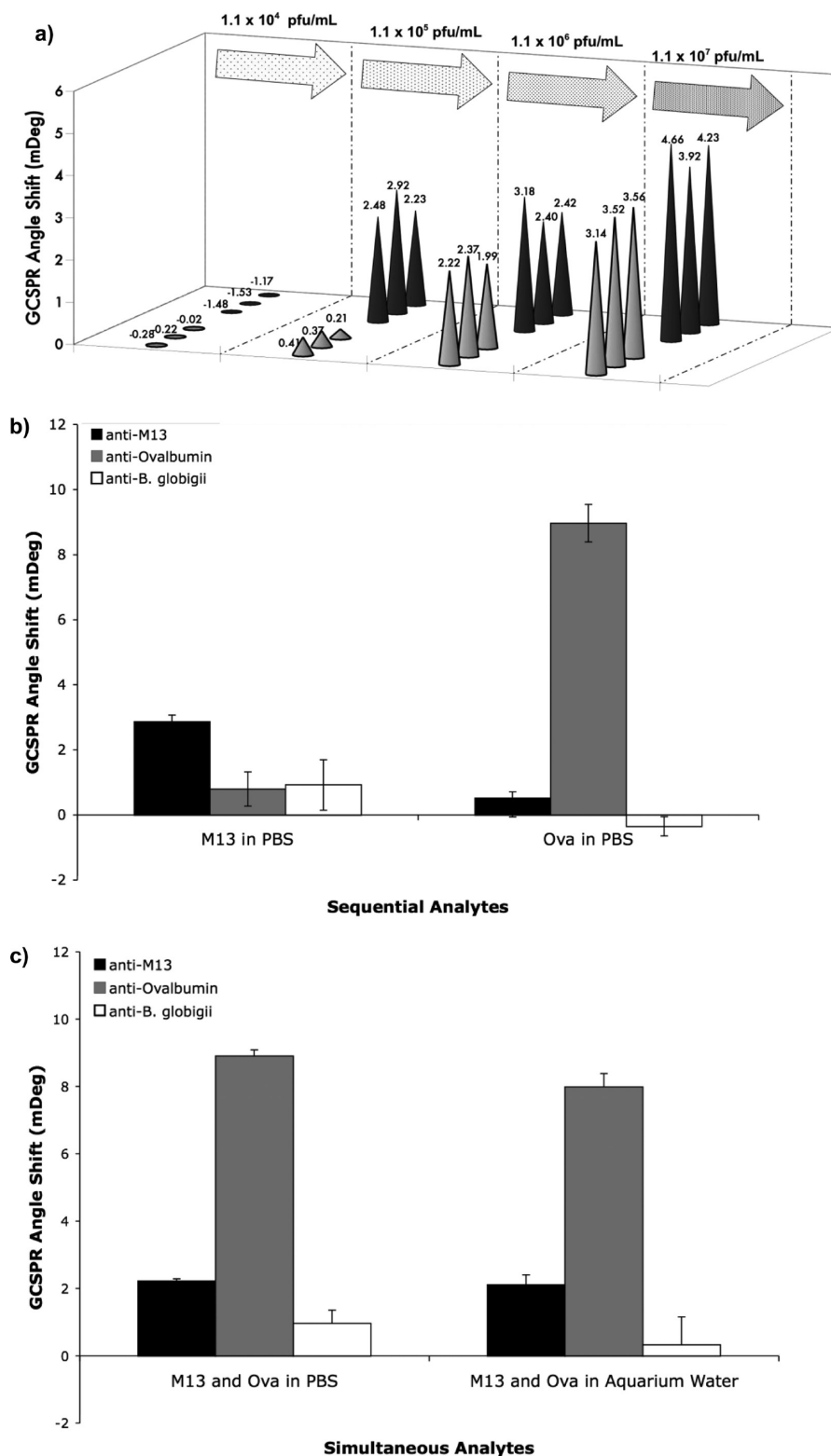
Figure 4. GCSPRI detection of viral particles at low concentrations and multianalyte detection in sterile and surrogate environmental samples by GCSPRI. (a) Anti-M13 antibody was immobilized on the sensor chip at concentrations of 0.5 (gray) and 1.0 mg/mL (black), each in triplicate. M13 bacteriophage samples (2 mL) of increasing concentrations ( \sim 10^4 , 10^5 , 10^6 , and 10^7 PFU/mL) were recirculated across the chip in succession, each for 20 min with a 10 min PBS wash in between to regenerate a baseline. (b) Anti-ovalbumin, anti-M13, and negative control anti- B. globigii antibodies (each at 1 mg/mL) were all three immobilized on three separate sensor chips. A 2 mL sample of M13 ( 10^6 PFU/mL) in PBS was flowed over the first chip for 20 min (left group). A 2 mL sample of ovalbumin (Ova) (20 \mu g/mL) in PBS was then delivered to the same chip (right group). (c) A 2 mL sample containing both 20 \mu g/mL ovalbumin and M13 ( 10^6 PFU/mL) mixed in PBS was flowed over the second chip (left group). Identical concentrations of ovalbumin and M13 were diluted in 2 mL of freshwater fish aquarium water and delivered to the third chip (right group).
