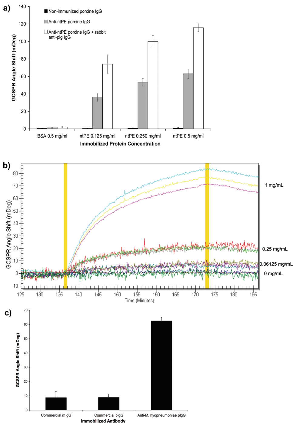
Figure 2. Specific GCSPRI detection of soluble analytes. (a) Triplicate spots of ntPE were immobilized on a sensor chip and the chip was exposed to a series of IgG antibodies. A 1:100 dilution of IgG from nonimmunized pig sera elicited a negligible GCSPRI angle shift (black bars). Subsequent flow of anti-ntPE IgG resulted in GCSPRI angle shifts at ntPE target ROIs only (gray bars). Next, an anti-porcine IgG secondary antibody (1:500 dilution) passed over the same surfaces caused a further increase in GCSPRI angle shifts (white bars). (b) Total protein from M. hyopneumoniae was diluted in 1% Stabilcoat (Surmodics) and immobilized on a sensor chip at the indicated concentrations, each in triplicate. After blocking (10% Superblock), anti- M. hyopneumoniae pIgG (162.5 \mu\text{g}/\text{mL} ) was flowed over the chip, followed by an Fc-specific goat anti-porcine IgG antibody (10 \mu\text{g}/\text{mL} ). The SPR response curve shows the GCSPRI angle shift resulting from anti-porcine IgG secondary antibody binding to captured anti- M. hyopneumoniae pIgG plotted as a function of time. (c) Purified IgG antibodies (500 \mu\text{g}/\text{mL} ) from naïve or immunized animals were immobilized in triplicate on the sensor chip. After blocking (10% Superblock), total protein from M. hyopneumoniae (100 \mu\text{g}/\text{mL} ) was delivered to the chip.
