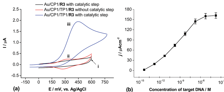
Figure 5. (a) Cyclic voltammograms obtained at a scan rate of 100 mV s -1 at the Au/CP1/TP1/R3 electrode for a 50 nM solution of TP1 target sequence with 2.5 mM DEA (iii) and without DEA (ii) in tris-HCl buffer solution. Curve (i) shows the control voltammogram obtained for the Au/CP1/R3 electrode. (b) Dependence of the oxidation current density on the TP1 concentration at the Au/CP1/TP1/R3 electrode.
