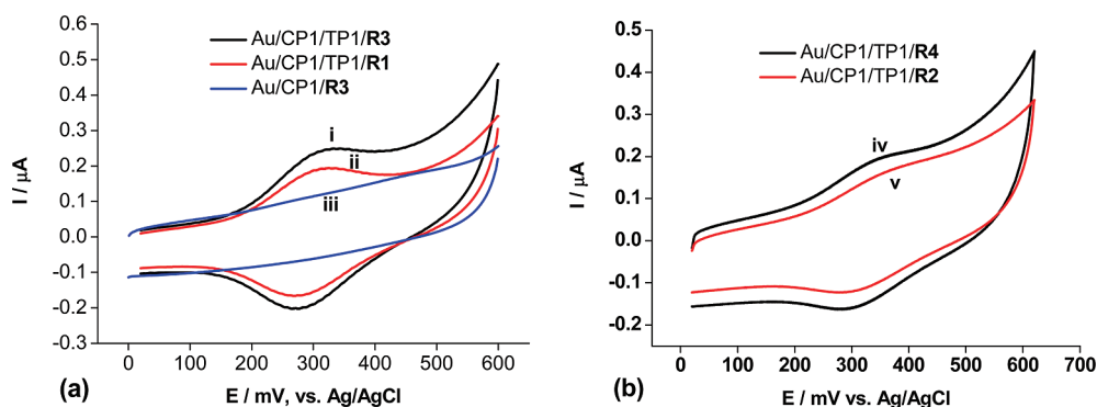
Figure 1. Cyclic voltammograms obtained at a scan rate of 100 \text{ mV s}^{-1} at (a) R1 - and R3 -functionalized and (b) R2 - and R4 -functionalized electrodes when 160 nM TP1 was hybridized to the thiolated ss-DNA probe in a 100 mM tris-HCl (pH 7.4) buffer solution.
