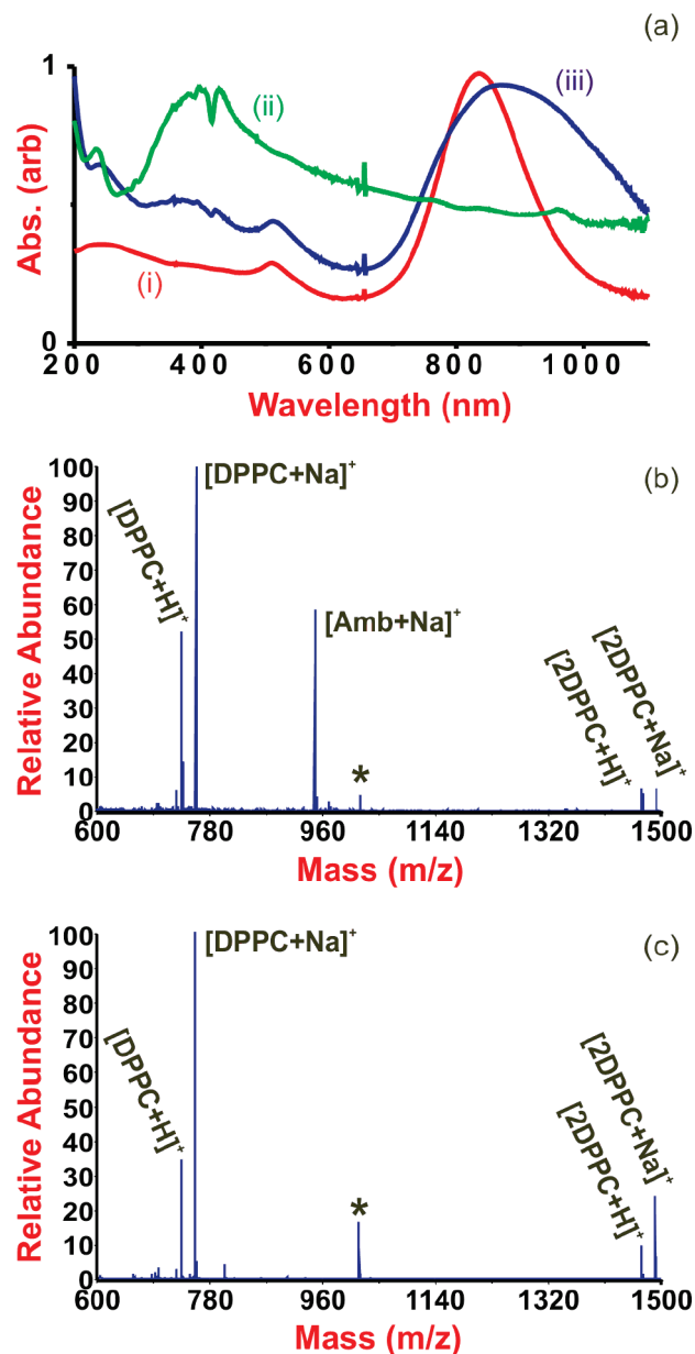
Figure 2. Capture of amphotericin B (AmB) with lipid-capped AuNRs followed by label-free detection using UV–vis spectroscopy and MALDI-MS. (a) UV–vis spectra of (i) lipid-capped AuNRs, (ii) a 10 \mu M solution of AmB, and (iii) a solution of the AmB–AuNR complex. (b) MALDI-MS mass spectrum of an AmB–AuNR complex after AmB was captured from a 1 \mu M AmB solution. (c) MALDI-MS mass spectrum of lipid-capped AuNRs. In (b) and (c), the peak labeled with an asterisk (*) was identified as a CTAB–DPPC complex by MS/MS.
