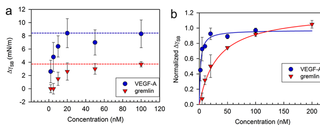
Figure 4. Nanomechanical study of the binding of VEGF-A and gremlin to surface immobilized sVEGFR2. (a) Representative \Delta\gamma_{\text{SB}} binding isotherms of VEGF-A (blue \bullet ) and gremlin (red \blacktriangledown ) with sVEGFR2 immobilized onto a 100 nm dextran-coated gold surface obtained by CONAMORE. The differential solid–solution interfacial tension, \Delta\gamma_{\text{SB}} , is referred to the BSA solution. Data points are the mean of three droplets deposited on the same chip; the error bars represent the SD of the mean. (b) Normalized \Delta\gamma_{\text{SB}} binding isotherms (same legend as in the previous caption). Data points are the overall mean of two replicate experiments conducted on different chips; the error bars represent the SD of the mean.
