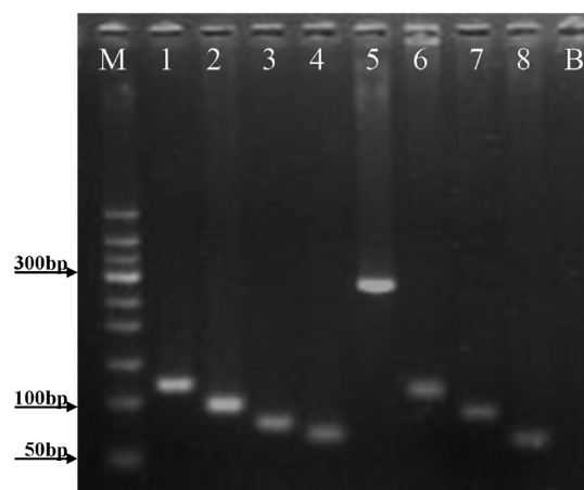
Figure 1. PCR amplification of target DNA fragments from eight food allergens. Lanes: M, 50 bp DNA Ladder marker; 1, soybean amplification with lectin gene (118 bp); 2, wheat amplification with gliadin gene (96 bp); 3, peanut amplification with Ara h 3 gene (78 bp); 4, cashew amplification with Ana o3 gene (67 bp); 5, beef amplification with mitochondrion DNA (271 bp); 6, shrimp amplification with 16S rRNA (109 bp); 7, fish amplification with 16S rRNA (86 bp); 8, chicken amplification with mitochondrion DNA (62 bp); B, blank control (ddH 2 O).
