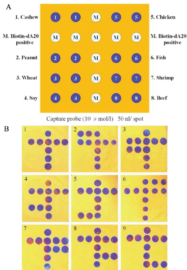
Figure 3. Food allergen detection on a chip with capture probes spotted by a computer-controlled dispenser. Each spot comprised 50 nL of 10 \mu mol/L probe solution and was printed in the order shown in (A). M, biotin-dA20 (positive control and marker); spot 1, Ana o3 gene (cashew); spot 2, Ara h 3 gene (peanut); spot 3, gliadin gene (wheat); spot 4, lectin gene (soybean); spot 5, mitochondrion DNA gene (chicken); spot 6, 16S rRNA (fish); spot 7, 16S rRNA (shrimp); spot 8, mitochondrion DNA (beef). (B) Detection of the food allergen-specific genes on thin-film biosensor chips: 1, blank control (ddH 2 O); 2, cashew; 3, peanut; 4, wheat; 5, soybean; 6, chicken; 7, fish; 8, shrimp; 9, beef.
