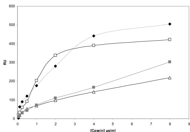
Figure 2. Effect of casein micelle concentration (in \mu g/mL) on the level of interaction between the casein micelle and monoclonal antibodies \alpha_{s1} -casein (f93–111) (◆), \alpha_{s2} -casein (f96–114) (■), \beta -casein (f76–93) (□), and \kappa -casein (f69–86) (△).
