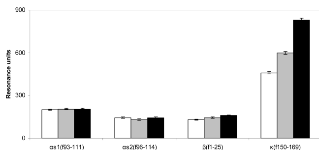
Figure 6. SPR signal (in resonance units) obtained on large (F1) (white bars), medium (F4) (gray bars), and small (F6) (black bars) casein micelles with monoclonal antibodies \alpha_{s1} -casein (f93–111), \alpha_{s2} -casein (f96–114), \beta -casein (f1–25), and \kappa -casein (f150–169).
