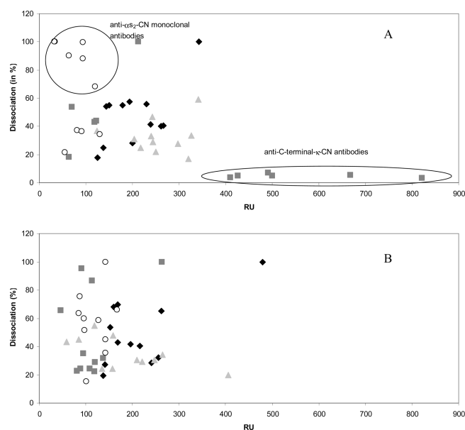
Figure 5. Dissociation of the antigen–antibody complexes versus the level of binding of the antigen on the captured anti- \alpha_{s1} - (▲), \alpha_{s2} - (○), \beta - (◆), or \kappa -casein (■) antibodies (in RU). The antigens were either casein micelle (A) or EDTA-dissolved caseins (B).
