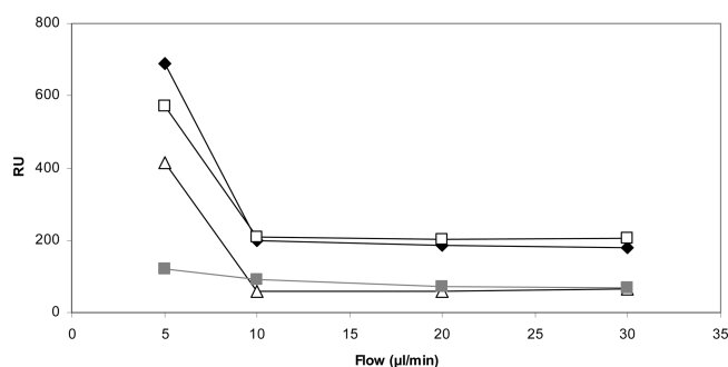
Figure 1. Effect of flow rate (in \mu L/min) on the level of interaction between the casein micelle and monoclonal antibodies \alpha_{s1} -casein (f93–111) (◆), \alpha_{s2} -casein (f96–114) (■), \beta -casein (f76–93) (□), and \kappa -casein (f69–86) (△).
