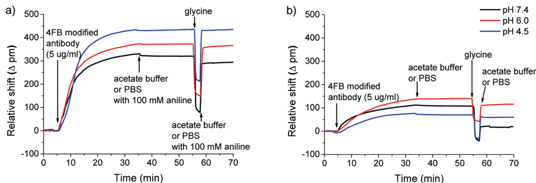
Figure 3. Real-time shifts in resonance wavelength from representative microrings upon covalent immobilization of anti(human thrombin) antibody onto the sensor surfaces at three different pHs and in the presence (a) and absence (b) of 100 mM aniline. In each trace, the sensors were initially incubated in buffer (with or without aniline, respectively) at a flow rate of 30 \mu\text{L}/\text{min} and a 5 \mu\text{g}/\text{mL} solution of 4FB-modified antibody with or without 100 mM aniline was flowed for 30 min. After switching back to the original buffer for 20 min, noncovalently attached antibody was removed with a low pH (pH 2.2) glycine buffer rinse. The sensors were then returned to the respective buffer at t = 57 min to determine the residual net shift corresponding to the amount of covalently immobilized antibody.
