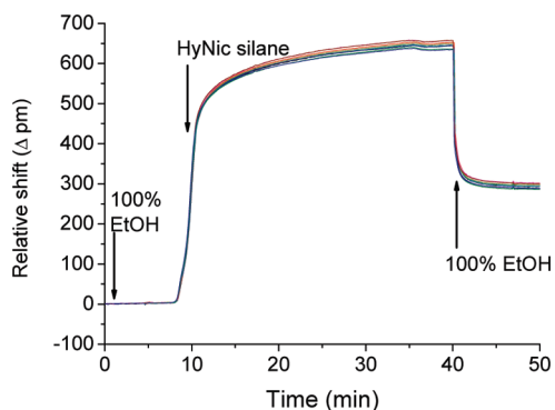
Figure 2. Real-time monitoring of the shift in resonance wavelength for ten microrings within the same sample flow chamber during organic modification via reaction with HyNic silane. The chamber was initially filled with 100% ethanol and a solution of 1 mg/mL HyNic silane in 95% EtOH and 5% DMF introduced under flow (5 \mu L/min) at t = 8 min. After 30 min, the HyNic silane was flushed from the chamber and microrings returned to 100% ethanol. The residual wavelength shift corresponds to immobilized HyNic silane.
