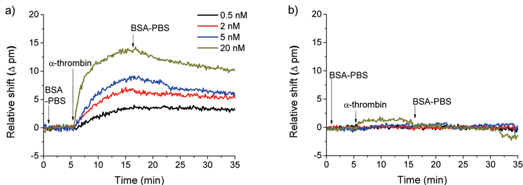
Figure 4. Time-resolved response from human \alpha -thrombin binding to microrings modified with anti(human thrombin) antibody at pH 7.4 in the presence (a) and absence (b) of 100 mM aniline. The microrings are initially in BSA–PBS buffer and thrombin is introduced at t = 5 min. Thrombin is then introduced and incubated for 10 min, after which BSA–PBS buffer is flowed to observe antigen dissociation. The remaining antigen–antibody interactions on the surface are then disrupted via exposure to a low pH (pH 2.2) glycine buffer for 2 min (not shown) to regenerate the sensor for subsequent detection experiments.
