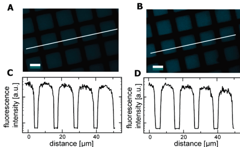
Figure 3. Fluorescence images of the (a) electron-beam-patterned and (b) X-ray-patterned PSA monolayers on diamond after reaction with the N,N' -didansyl-L-cysteine dye. (c,d) Cross sections along the white lines shown in (a) and (b), respectively. The dynamic range of fluorescence intensity corresponds to 2 orders of magnitude. The white scale bar represents 10 \mu\text{m} .
