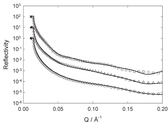
Figure 4. Reflectivity profiles for 1× bilayer (O), 2× bilayer (Δ), and 3× bilayer (□) of phthalocyanine at the silicon/D 2 O interface. The solid lines show the best fit to the data. The profiles are shifted by a factor of 10 for the purpose of clarity.
