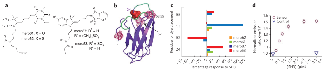
Figure 3 | Screening for responsive sensor variants, selecting dye and site for dye labeling. (a) Structures of the environmentally sensitive merocyanine dyes tested on the monobody. (b) Ribbon representation of the active-state binder 1F11 (based on published FN3 domain crystal structure PDB 1FNA). Residues 2, 24, 52, 53 and 55, where cysteine was incorporated for dye attachment and testing, are shown as space-filling side chains. Ala24, labeled in red, marks the position of dye attachment in the final merobody biosensor. The putative target-binding loops are shown in cyan. (c) Ratiometric fluorescence response (dye emission/mCerulean emission) of the various combinations of mero dyes and residues labeled. (d) Titration showing how the normalized emission ratio of mero53/mCerulean for the biosensor or control (0.5 \mu M) changes with increasing c-Src SH3. The control sensor has a P80A mutation in the FG binding loop of 1F11.
