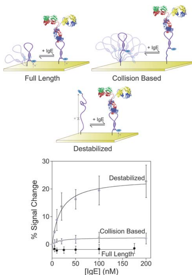
Fig. 5 Neither the full-length anti-IgE aptamer nor a construct modified via the addition of a 10-base polythymine linker to increase flexibility supports efficient E-AB signaling. In contrast, a destabilized sequence (through point mutation) supports at least modest E-AB gain. The destabilized aptamer produces a signal change of 20% at saturating IgE concentrations (200 nM) with an apparent affinity of 18 \pm 3 nM.
