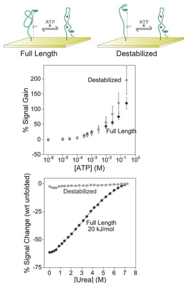
Fig. 2 Both the full-length anti-ATP aptamer (top left) and a destabilized sequence (top right) support efficient E-AB signaling (middle). The destabilized sequence produces a gain (relative signal change in the presence of target) of 190%, which is slightly greater than the 130% observed for the full-length aptamer. Urea denaturation curves (bottom) performed on electrode-bound aptamers indicate that the full-length sequence is folded in the absence of ATP. The destabilized construct, in contrast, appears to be unstructured in the absence of target. Reported error bars reported here in and in the following figures represent the standard deviation of measurements taken from at least three independently fabricated sensors.
