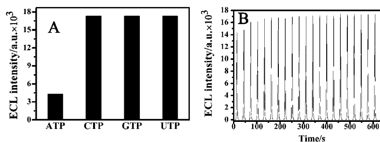
Fig. 8 (A) ECL signal specificity of aptasensor towards ATP and its three analogues CTP, GTP and UTP. The aptasensor was incubated with 50 \mu\text{g mL}^{-1} ATP, CTP, GTP or UTP solution respectively for ECL detection. (B) ECL-time curve of QDs/cDNA/probe/Au electrode under continuous cyclic voltammetry scan. The electrolyte was 5 mL PBS + solution containing 0.1 M \text{K}_2\text{S}_2\text{O}_8 and 0.1 M KCl. The voltage of the photomultiplier tube was 600 V and the scan rate 100 \text{ mV s}^{-1} .
