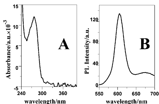
Fig. 3 UV (A) and PL (B) spectra of the QDs in 0.1 M PBS (pH 7.4). The PL excitation wavelength was 360 nm.
