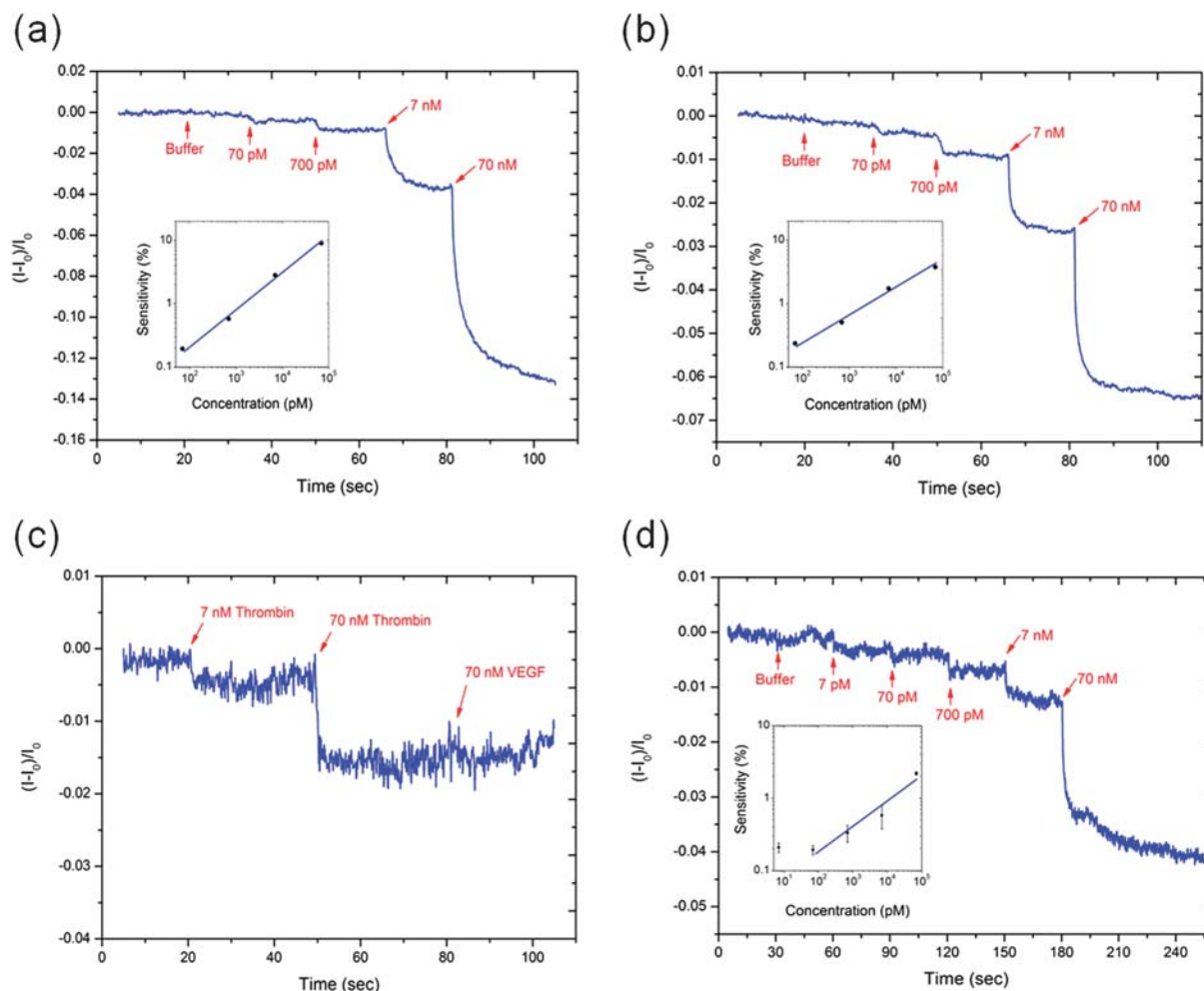
Fig. 4 Real-time electrical detection of proteins using thrombin DNA aptamer-functionalized SWNT-film FET biosensors: Real-time electrical detection for the nonspecific binding of (a) thrombin and (b) VEGF to the SWNT-COOH films. (c) Specific binding tests of thrombin molecules to the SWNT-film aptasensor after treatment with Tween 20. (d) Real-time electrical detection for the specific binding of thrombin molecules with increasing concentrations to the SWNT-film aptasensor. Insets show the sensitivity of the SWNT-film aptasensor with increasing protein concentrations on a log–log scale ( n = 4 ).
