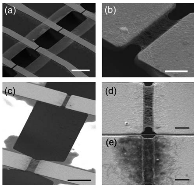
Fig. 2 SEM images of suspended SWNT-film arrays at the magnifications of (a) \times 400 (scale bar: 50 \mu\text{m} ) and (b) \times 5,000 (scale bar: 5 \mu\text{m} ). (c) SEM image of suspended SWNT-films with a different channel length (scale bar: 20 \mu\text{m} ). SEM images of aptamer functionalized SWNT-films (d) before and (e) after thrombin binding (scale bars: 5 \mu\text{m} ).
