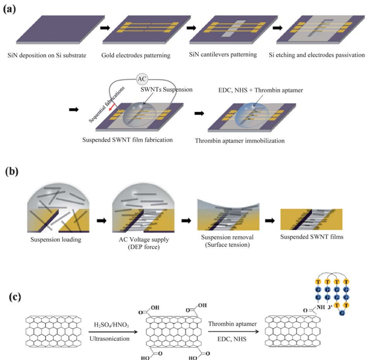
Fig. 1 Schematic representations for (a) the fabrication of thrombin aptamer functionalized SWNT-film field effect transistor (FET) biosensors, (b) the preparation of suspended SWNT-films by dielectrophoresis and surface tension, and (c) the surface modification of SWNT in a strong acid to introduce carboxyl groups and the following covalent immobilization of thrombin aptamers by amide bond formation using 1-ethyl-3-[3-(dimethylamino)propyl]carbodiimide (EDC) and N-hydroxysulfosuccinimide (sulfo-NHS).
