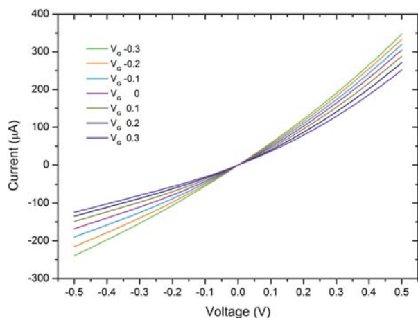
Fig. 3 Electrical characteristics of suspended SWNT-films at various electrolyte gate voltages from -0.3 V to 0.3 V.
