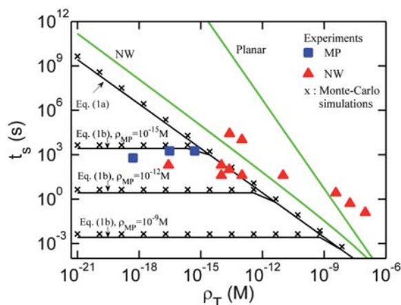
Fig. 2 Settling time as a function of target molecule density ( N_s = 1 ). Analytic solutions are shown as solid lines while Monte-Carlo simulation results are shown as 'x' symbols. The settling time for NW (radius 50nm, length- 1\mu\text{m} , time to capture N_s = 3 molecules per NW) and planar sensors, based on ref. 2, are also plotted. The simulation parameters are: D = 10^{-6}\text{cm}^2/\text{s} , a_0 = 0.5\mu\text{m} . The solid squares represent experimental data using MP sensors (ref. 5–7) while the solid triangles represent experimental data using NW sensors from various groups (ref. 14–19). The theoretical results on the performance limits of planar, NW, and MP sensors can also be accessed through an online simulation tool, Bio-SensorLab . 20
