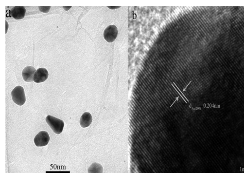
Fig. 2 (a) TEM and (b) HRTEM image of the GNPs–GNSs nanocomposite.
