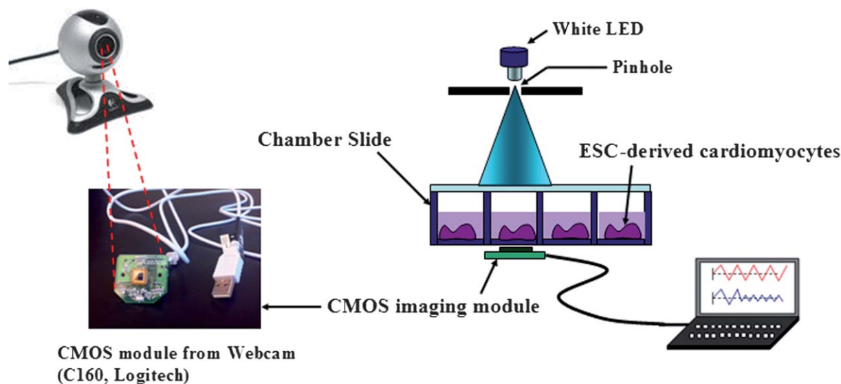
Fig. 1 Schematic of the experimental setup. ESC-derived cardiomyocytes were plated on a chamber slide. The white LED and a pinhole combination was used as a light source for imaging the beating cardiomyocytes. The real-time beating rates of the cardiomyocytes were measured using the CMOS imaging module which controlled by an image processing program.
