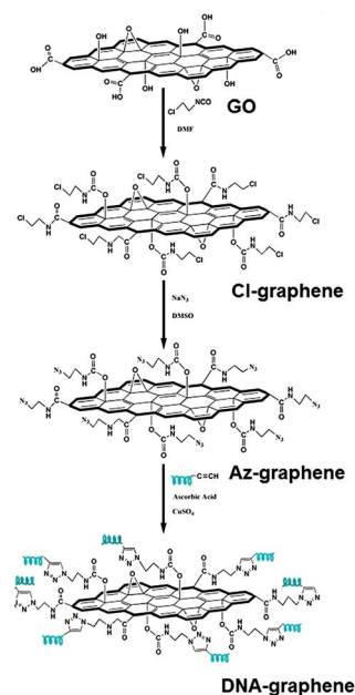
Fig. 1 Schematic representation of the synthesis route of DNA–graphene conjugates.
