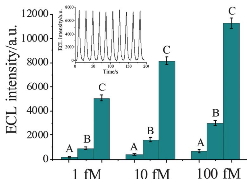
Fig. 6 Comparison of ECL signal with a series of target DNA ( 1.0 \times 10^{-15} , 1.0 \times 10^{-14} , and 1.0 \times 10^{-13} M): the target DNA (C), one-base mismatched DNA (B), and completely mismatched target DNA (A). Error bars showed the standard deviations of measurements. The inset was the stabilization of ECL emission of 1.0 \times 10^{-13} M target DNA on NPG-electrode in 10 mM Tris-HCl buffer (pH 7.4) containing 0.1 M K_2S_2O_8 and 0.1 M KCl, under continuous cyclic scans between -0.8 to -1.8 V for 10 cycles. Scan rate, 100 \text{ mV s}^{-1} .
