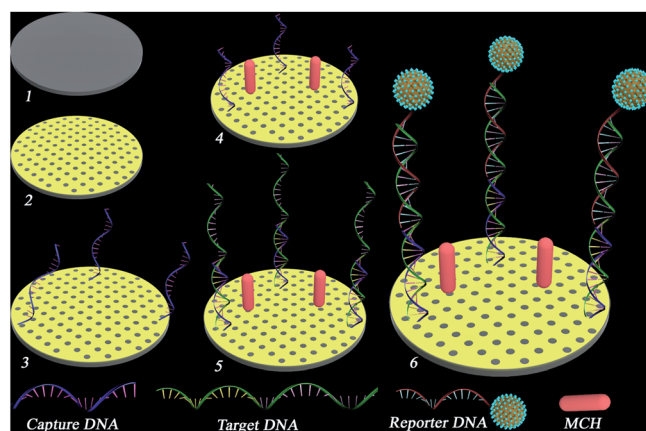
Fig. 1 Schematic representation of the fabrication of the DNA biosensor (1) GCE, (2) GCE assembled with NPG, (3) after immobilization of capture DNA (S 1 ), (4) after blocking with MCH, (5) hybridization with target DNA (S 2 ), and (6) hybridization with the PdCu@CNCs labeled reporter DNA (S 3 ).
