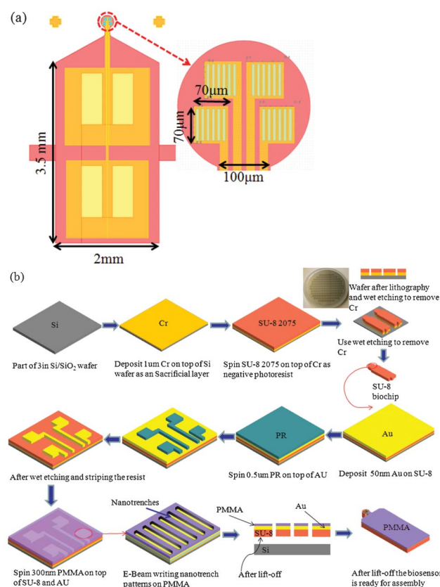
Fig. 2 (a) Design of the biosensor microchip: Holder with contact pads (left) and four separated biosensor regions (right) on a 250-μm-diameter biosensor. (b) Process schematic of the biosensor microchip's fabrication.
