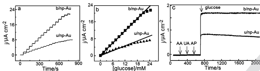
Fig. 5 Current responses of GOx/bimodal np-Au and GOx/uniform np-Au on successive addition of 1.5 mM glucose into a stirring PBS (50 mM, pH 7.0), applied potential: -0.3 V (a); plots of currents vs. glucose concentrations (b); current responses of the two GOx modified electrodes on the addition of AA ( \sim 0.1 mM), AP ( \sim 0.1 mM), UA ( \sim 0.02 mM), and glucose (1.5 mM).
