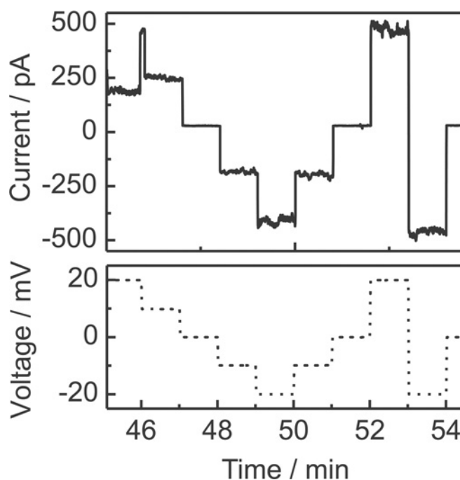
Figure 12 Formation of stable lesions in an asymmetric LPS/PL bilayer
