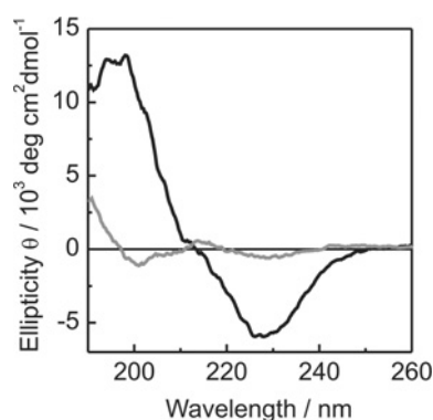
Figure 7 Secondary structures of NK-2 and NK11 analysed by CD spectroscopy
