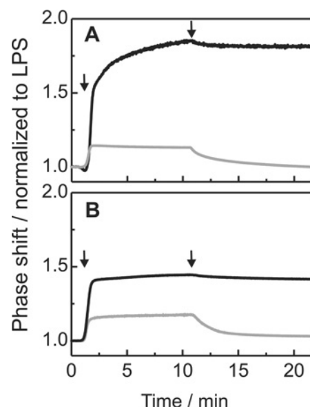
Figure 8 Binding of NK-2 and NK11 to LPS bilayers using SAW
