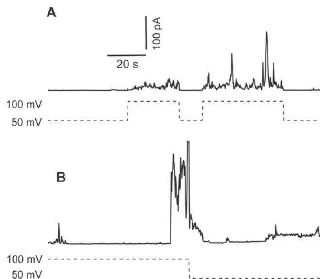
Figure 11 Formation of transient lesions in asymmetric LPS/PL bilayers
