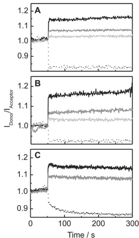
Figure 9 FRET spectroscopy of the insertion kinetics of NK-2 and NK11 into LPS bilayers
