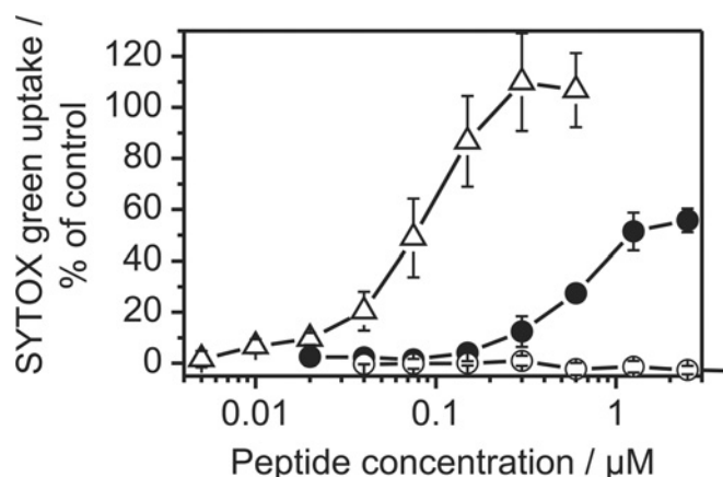
Figure 6 Permeabilization of bacterial membranes by AMPs
