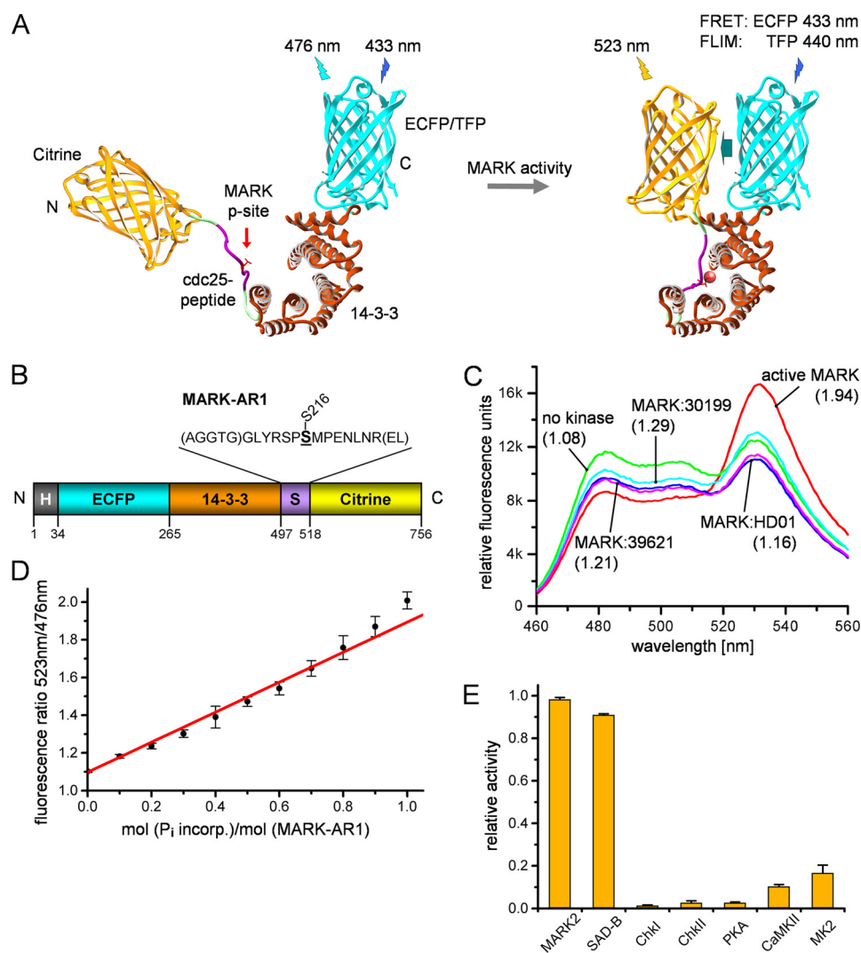
FIGURE 6. Schematic diagram and in vitro properties of the MARK activity reporter. A , a MARK-specific target peptide (derived from residues 210–223 of Cdc25C, GLYRSPMPENLNR) containing the phosphorylation site Ser-216 is fused via linkers (in parentheses) to 14-3-3 protein (brown), with ECFP and YFP (citrine) as a FRET pair at both ends. Upon phosphorylation, the target sequence binds into the pocket of 14-3-3, which closes up and generates an enhancement of the FRET signal. TFP, teal fluorescent protein. B , shown is a bar diagram of the MARK activity reporter (MARK-AR1). For in vitro studies, the protein was labeled with a polyhistidine tag (H; gray), allowing simple and rapid purification. N and C denote the N and C termini of the construct. C , shown is a wavelength scan of the unphosphorylated and phosphorylated MARK-AR1. The fluorescence of the unphosphorylated MARK-AR1 shows a maximum at 476 nm (green curve), whereas the maximum for the phosphorylated protein is shifted to 523 nm due to FRET (red curve). The inhibitors HD01 (blue curve), 30199 (cyan curve), and 39621 (pink curve) prevent the phosphorylation by MARK. Inhibitor concentrations were 5 \mu M (HD01) and 20 \mu M (30199 and 39621). Shown in parentheses is the ratio of the emission at 523 nm to the emission at 476 nm. D , the ratio of the emission at 523 nm to the emission at 476 nm can be taken as a measure of activity, as it shows a linear relationship to the phosphorylation of the activity reporter. The x axis displays the amount of incorporated radioactively labeled phosphate into the MARK-AR1, whereas the y axis shows the corresponding emission ratios, ranging from 1.08 (no phosphorylation) to 1.94 (complete phosphorylation of the target site). E , MARK-AR1 can be phosphorylated by MARK and SAD-B. Other kinases reported to phosphorylate Cdc25C cannot effectively phosphorylate this activity reporter.
