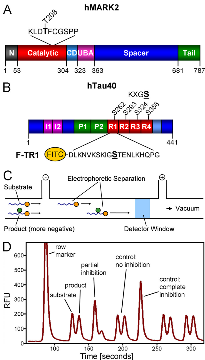
FIGURE 1. Bar diagrams of MARK and hTau40. A, shown is a bar diagram of MARK2 as a representative for the four mammalian MARK isoforms. All MARKs share a similar architecture with high homologies in the catalytic domain, common docking site (CD), ubiquitin-associated domain (UBA), and kinase-associated domain. Variations are found mostly in the spacer domain and the N-terminal header (N). The activation loop in the catalytic domain contains a critical threonine (Thr-208 in MARK2, indicated above), whose phosphorylation by MARK or LKB1 is required for full activity. By contrast, phosphorylation of Ser-212 by GSK3 \beta is inhibitory. B, shown is FITC-labeled peptide derived from the first repeat of the Tau protein containing the residue Ser-262 (underlined) that is phosphorylated by MARK isoforms. C, shown is a schematic drawing of the separation of substrate and product by capillary electrophoresis on the LabChip™. The chip holds 12 parallel channels. D, shown is an example of a chromatogram showing substrate and product peaks of sample with no inhibition or partial and complete inhibition. RFU, relative fluorescence units.
