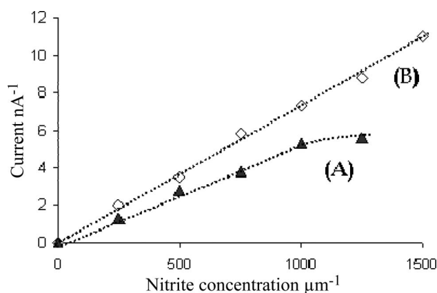
Figure 9. Nitrite biosensor. Calibration curves using S. nitritireducens at 20^\circ\text{C} (A) and 30^\circ\text{C} (B). (Adapted from Larsen et al. 2000.)
