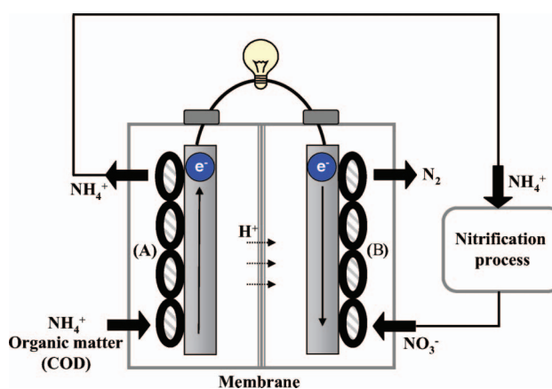
Figure 8. 'Nitrogen loop system' for the combined removal of carbon and nitrogen (Virdis et al. 2008). Organic matter containing carbon is oxidized on the bioanode (A). The resulting effluent is then treated in an external aerobic nitrification process converting ammonium into nitrate. The wastewater is finally diverted to the biocathode where nitrate reduction occurs (B).
