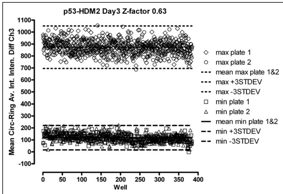
Fig. 5. Three-day assay signal window and Z-factor determination. U-2 OS cells were coinfectd with the p53-hDM2 protein-protein interaction biosensor adenoviruses, seeded at 2,500 cells per well in 384-well Greiner collagen-coated assay plates, and cultured overnight at 37°C, 5% CO 2 , and 95% humidity as described earlier. Two maximum control plates (max plate 1 ◇, max plate 2 ○) were then treated with 0.5% dimethyl sulfoxide and 2 minimum control plates (min plate 1 □, min plate 2 △) were treated with 10 μM Nutlin-3 for 90 min prior to fixation with 3.7% formaldehyde containing 2 μg/mL Hoechst 33342. Images were acquired on the ArrayScan V TI platform and analyzed with the molecular translocation image analysis algorithm as described for Figure 2. The mean circle ring average intensity difference in channel 3 (MCRAID-Ch3) data was used as the primary indicator of the interactions between p53 and hDM2. Three independent experiments of 2 full 384-well plates each of maximum and minimum plate controls were conducted on 3 separate days (Table 1). A scatter plot of the hDM2-red fluorescent protein MCRAID-Ch3 signals from the 2 full 384-well plates each of maximum ( n = 768 ) and minimum ( n = 768 ) controls performed on day 3 is presented.
