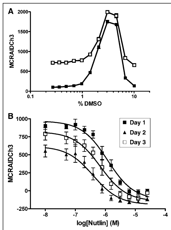
Fig. 4. Dimethyl sulfoxide (DMSO) tolerance and Nutlin-3 \text{IC}_{50} determinations. (A) DMSO tolerance. U-2 OS cells were coinfectd with the p53-hDM2 protein-protein interaction biosensor (PPIB) adenoviruses, seeded at 2,500 cells per well in 384-well Greiner collagen-coated assay plates, and cultured overnight at 37°C, 5% \text{CO}_2 , and 95% humidity as described earlier. Cells were then treated with 0.5% DMSO ( \square ) or 10 \mu\text{M} Nutlin-3 ( \blacksquare ) at the indicated concentrations of DMSO for 90 min prior to fixation with 3.7% formaldehyde containing 2 \mu\text{g}/\text{mL} Hoechst 33342. (B) Nutlin-3 \text{IC}_{50} determinations from 3 independent experiments. U-2 OS cells were coinfectd with the p53-hDM2 PPIB adenoviruses, seeded at 2,500 cells per well in 384-well Greiner collagen-coated assay plates, and cultured overnight at 37°C, 5% \text{CO}_2 , and 95% humidity as described earlier. Cells were then treated with the indicated concentrations of Nutlin-3 for 90 min prior to fixation with 3.7% formaldehyde containing 2 \mu\text{g}/\text{mL} Hoechst 33342. Images were acquired on the ArrayScan V Hi platform and analyzed with molecular translocation image analysis algorithm as described for Figure 2. The mean circle ring average intensity difference in channel 3 (MCRAID-Ch3) data was used as the primary indicator of the interactions between p53 and hDM2. The data are presented as the mean MCRAID-Ch3 values \pm SD from (A) n = 16 wells, (B) n = 16 wells at day 1, and n = 24 wells at days 2 and 3. For the \text{IC}_{50} determinations, the resulting nonlinear regression curves were plotted using the following sigmoidal dose-response variable slope equation: Y = \text{Bottom} + [\text{Top} - \text{Bottom}] / [1 + 10^{-(\text{LogEC}_{50} - X) \times \text{Hill slope}}] , using Graphpad Prism software 4.03. Data from a single representative experiment of 2 independent DMSO-tolerance experiments are presented in A, and the data from 3 independent \text{IC}_{50} experiments are presented in B. The \text{IC}_{50}\text{s} for the disruption of the p53-hDM3 PPIB were 1.196, 0.394, and 0.680 \mu\text{M} on days 1, 2, and 3, respectively.
