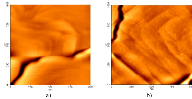
Figure 2. AFM micrographs ( 1000 \times 1000 \text{ nm}^2 , z scale 3 nm) of a) hydroxylated 3C-SiC. b) Corresponding APTES modified surfaces. Images taken in non-contact mode.
