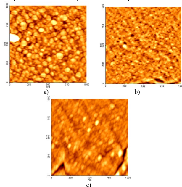
Figure 4. AFM micrograph (1000 X 1000 nm 2 , z scale 5 nm, non-contact mode) after myoglobin immobilization a) surface A (covalent immobilization and BSA blocking), b) surface B (non-covalent adsorption) and c) surface C (covalent immobilization and no BSA blocking).
