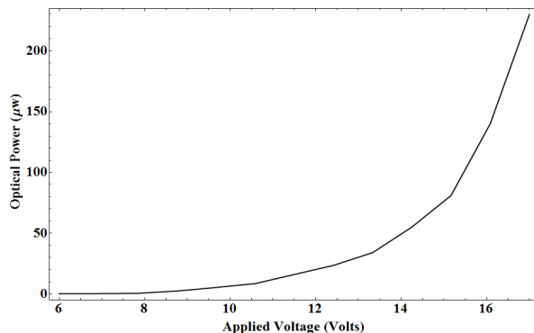
Fig 10. Plot of Optical power output versus Applied voltage.
