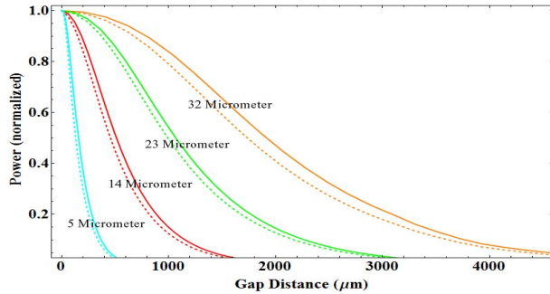
Fig. 7. Plot shows transmittance curves for different spot sizes, the dotted lines indicate combined mode, thick lines in the plot indicate fundamental mode the refractive index being 1.37.
