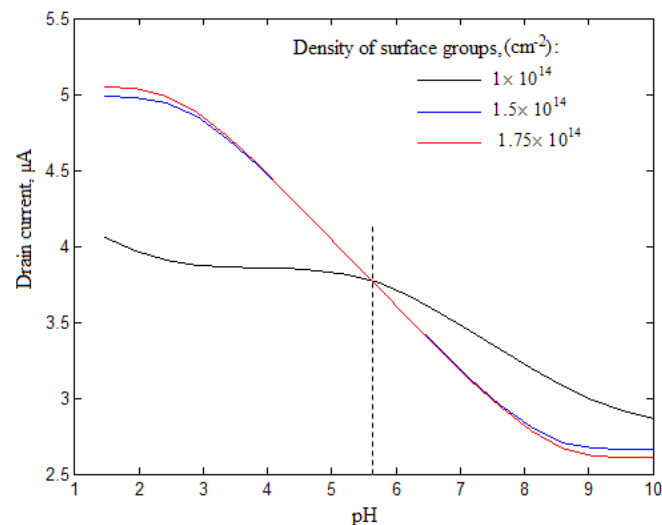
Figure 4. Graph illustrating the dependence of drain current on the pH of the solution and with different values of surface group density.
