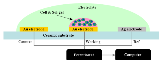
Fig. 1. Schematics of 3D cell based electrochemical biosensor. Cells mixed with sol-gel were spotted on the working electrode and gel-cells mixture was gelated on gold electrode.
