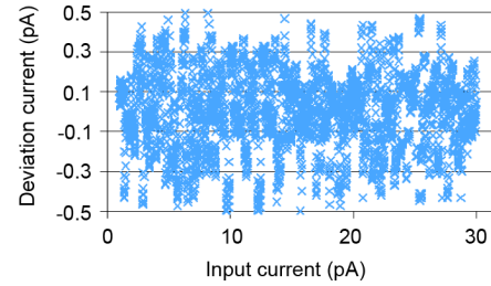
Fig. 11. The deviation between input current and measured current for 1 pA to 30 pA inputs at 20 Hz updating clock and gain=2 setting.
