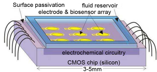
Fig. 1. Conceptual illustration of a CMOS circuit with on-chip electrode array and packaging for use in a liquid environment.
