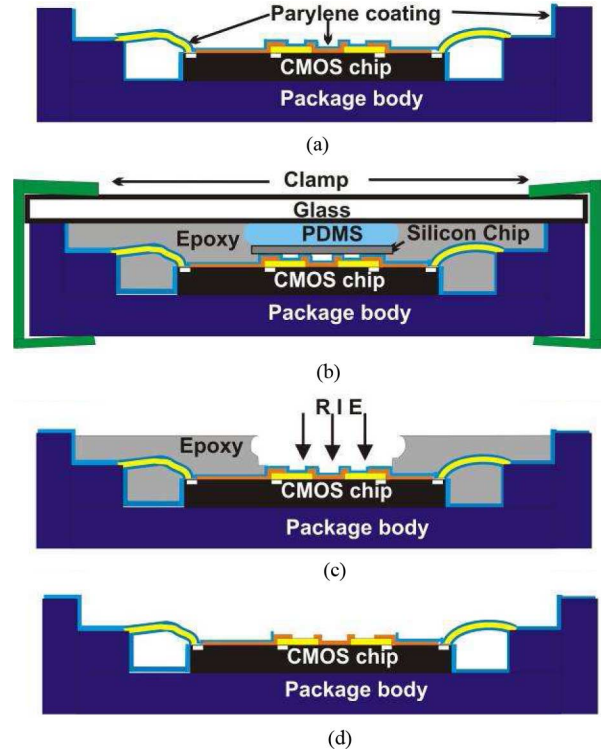
Fig. 9. Process flow of chip-in-package sealing for liquid environment. (a) Chip is wire-bonded to package and coated by 5 \mu\text{m} parylene. (b) A PDMS cylinder and silicon chip are attached to a glass slide and clamped to the package to cover the center of the CMOS chip before crystal adhesive is melted to fill the cavity. (c) Glass slide is detached and parylene is etched away by oxygen RIE. (d) Crystal adhesive removed to form final package with all non-electrode surfaces insulated.
