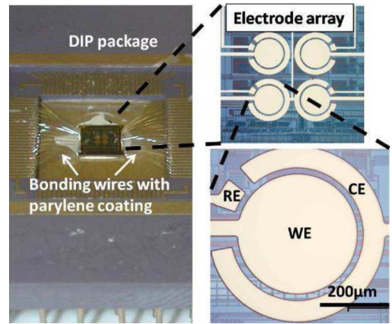
Fig. 12. Photograph of a CMOS biosensor array chip-in-package and close up views of the post-CMOS surface electrode array.
