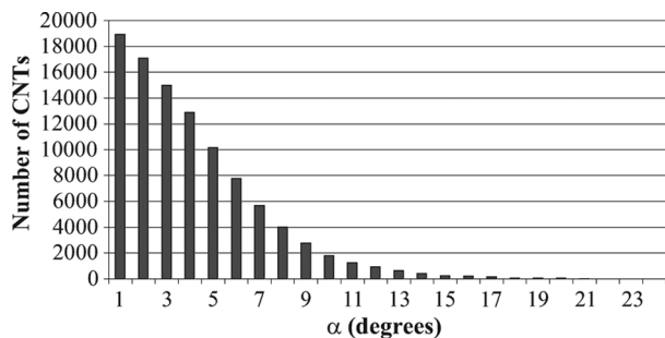
Fig. 5. Results from Monte Carlo simulation for the distribution of carbon nanotubes onto a flat surface.
