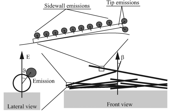
Fig. 4. Carbon nanotubes randomly organized onto the electrode surface and covered with proteins.
