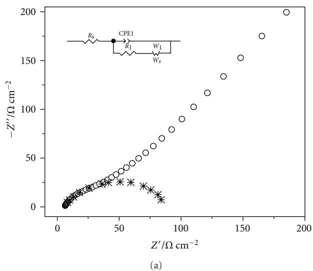
FIGURE 2: Typical Nyquist plots: (a) carbon nanotube paste electrode (60% w/w), (b) CNTs-AChE biosensor in 5.0 mM K_3[Fe(CN)_6] in 0.5 M KCl solution. Insert: the proposed Randle's model.
