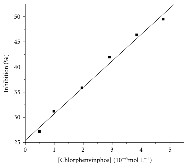
FIGURE 5: Analytical curve obtained with the CNTs-AChE biosensor for different concentrations of chlorphenvinphos in phosphate buffer pH 7.4 and 3.0 \times 10^{-3} \text{ M} AcSch. Cell temperature is 30^\circ \text{C} .
