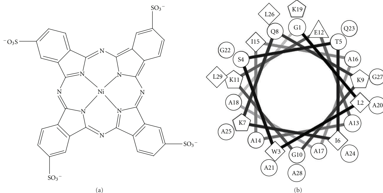
FIGURE 1: Chemical structures of materials used in LbL films: (a) nickel tetrasulfonated phthalocyanine (NiTsPc) and (b) amino acid sequence and helix-wheel plots of the antimicrobial peptide (DS 01) showing the amphiphilic character of the molecule.
